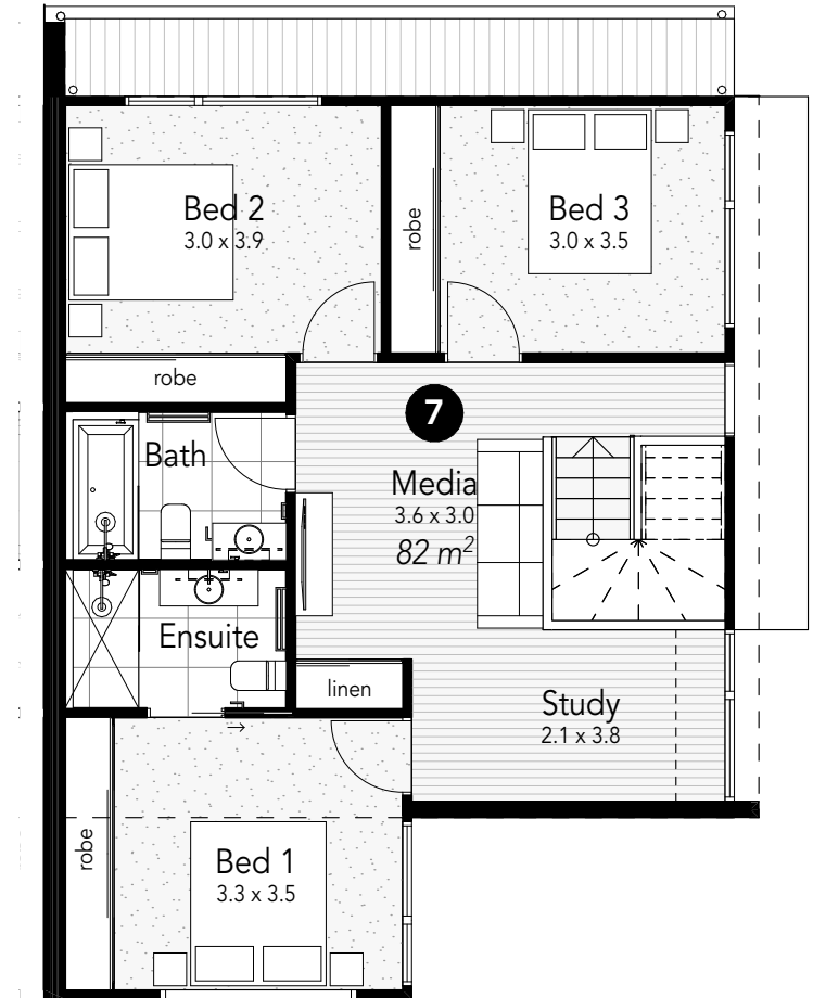
Upper Floor
